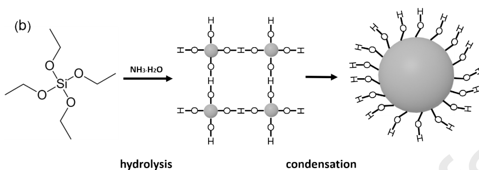
Figure1 : (a) Experimental set-up of the microfluidic mixer for (b) the continuous synthesis of \text{SiO}_2 particles.
