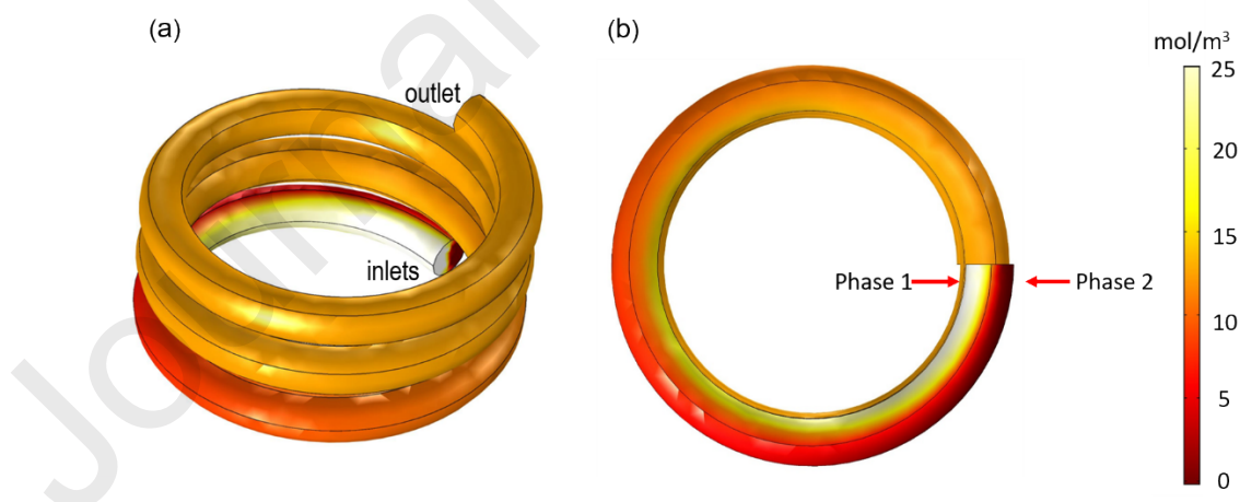
Figure 2. Simulation of the spiral microreactor. (a) A side perspective showing the microreactor with inlets and outlets. (b) a top view along the spiral axis to illustrate the two distinct phases that are introduced into the inlet. The concentration gradient represented by the colour gradient from white to red is shown in the colour bar. As the two phases move along the spiral, fast mixing occurs and the two phases merge into a single phase after one run. Here d_p is 0.8 mm, d_R = 6 mm, and the total flow rate is 400 \mu\text{L}/\text{min} .
