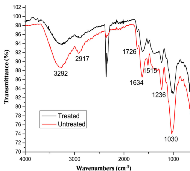
Fig. 3 FT-IR spectra of A. cepa root tip before and after interaction with \text{Al}_2\text{O}_3 NPs
